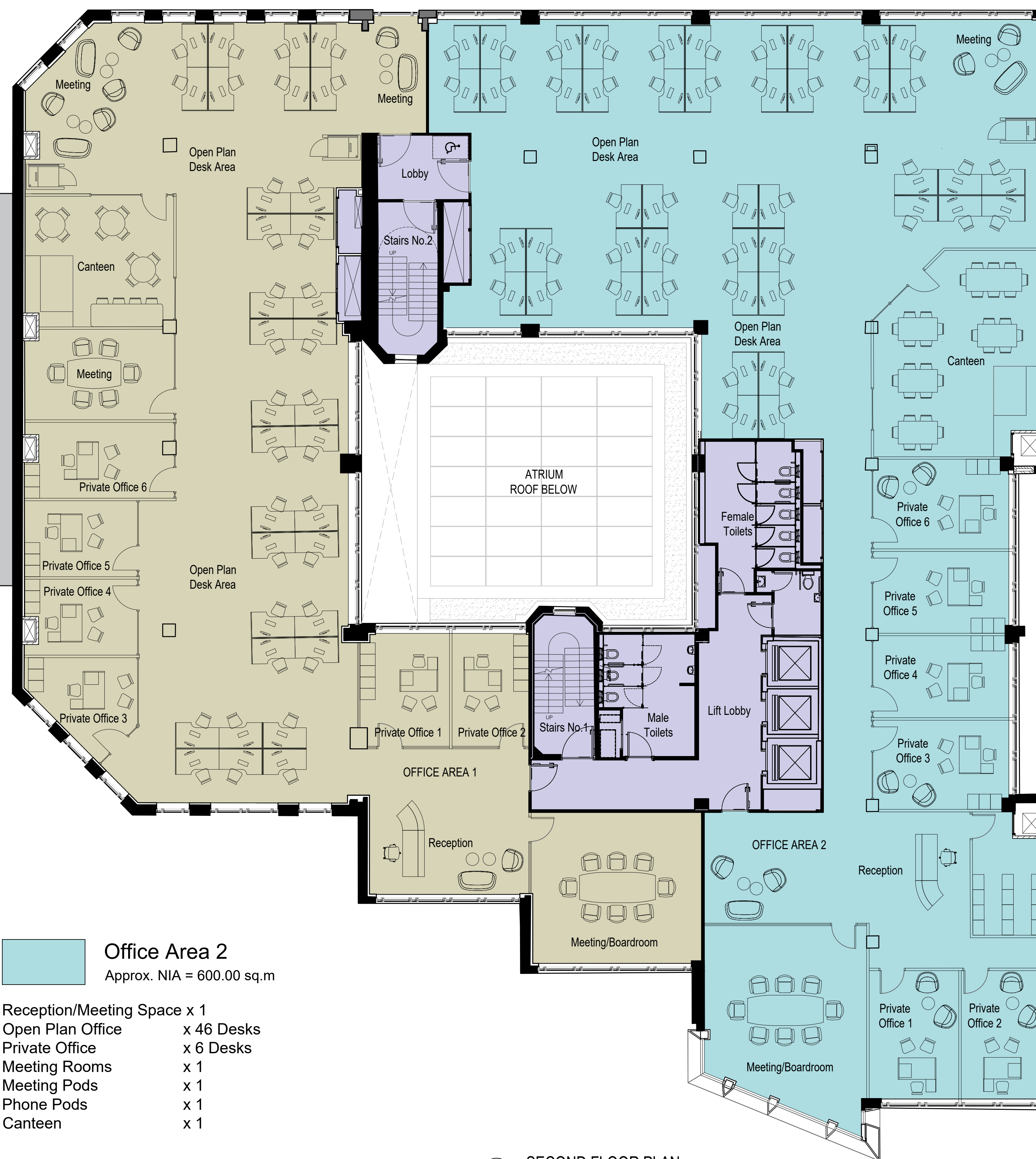
1 SECOND FLOOR PLAN 206 1:100 @ A1
